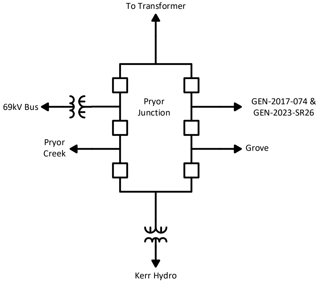
Figure 1: Point of Interconnection (POI INFORMATION) One-Line Diagram
